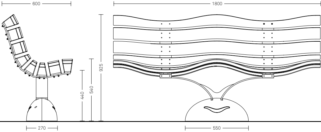
Panchina 2197.002 T 2197.300.002* T
