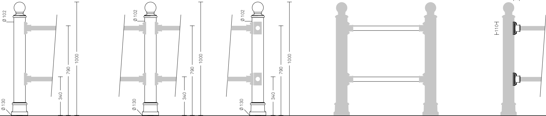
Railing – column 2971.050 M
