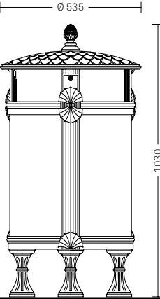
Layia 2270.000 M Alluminium and galvanized steel Capacity 50l
