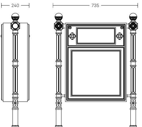
Scilla 2271.000 S2 M 2272.000 S1 M S2 opening on two sides S1 opening on one side Cast iron, aluminium and galvanized steel Capacity 31l
