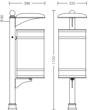
Melia – with cover 2275.001 B1 M 2275.101 B2 M B1 single basket B2 double basket Cast iron and galvanized steel Capacity 37l (single basket) and 74l (double basket)
