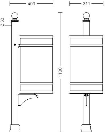
Melia 2275.000 B1 M 2275.100 B2 M B1 single basket B2 double basket Cast iron and galvanized steel Capacity 37l (single basket) and 74l (double basket)
