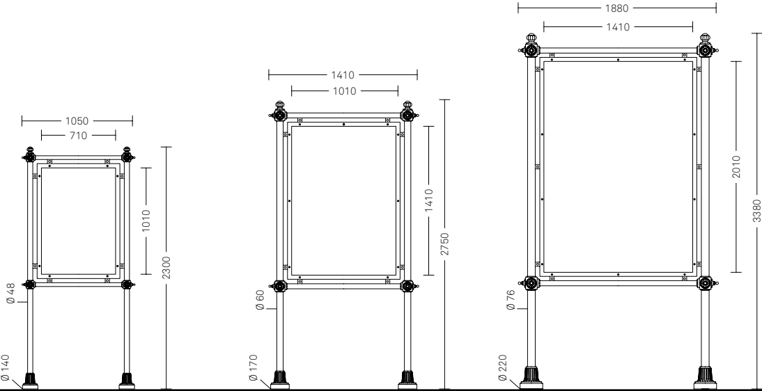
Portrait notice board 2291.000.500 M
