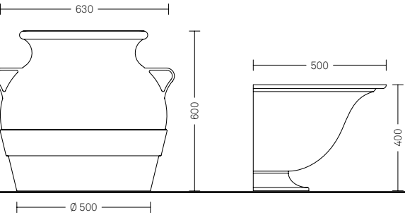
Layia 2212.000.001 T • Cast iron • Capacity 125l
