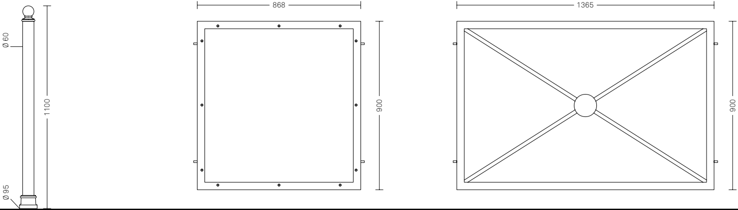
Railing – column 2970.000.003 M
