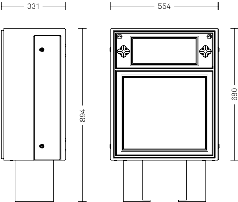
Scilla – switchboards 2272.000.005 M 2 lateral compartments that host switchboards (electric accessories not included) Cast iron, aluminium and galvanized steel Capacity 31l
