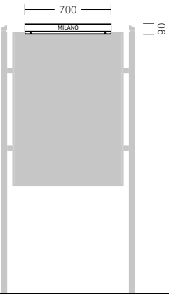
Coping 0002.298 Notice board accessory • Customizable text
