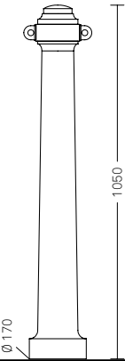
Bollard 2985.000 M 2985.001 R • Nodular cast iron
