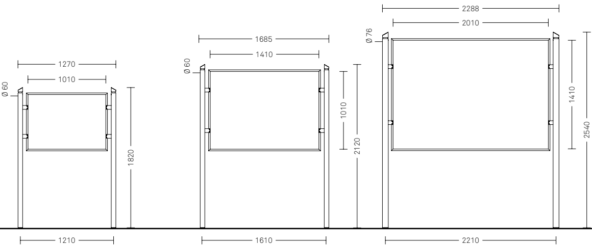
Landscape notice board 2298.100.010 M 2298.200.010 M 2298.300.010 M Small series • Galvanized steel • Aluminium panel Medium series • Galvanized steel • Aluminium panel Large series • Galvanized steel • Aluminium panel
