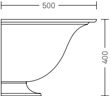
Salix – wall mounted 2203.001 T • Cast iron • Capacity 57l
